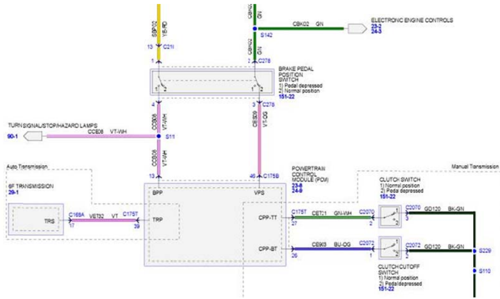
Figure 14: The brake pedal switch and electronic engine controls are wired into the PCM
